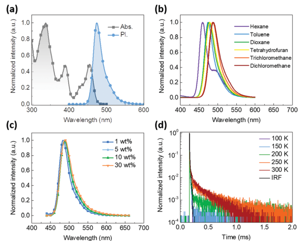
Fig. 3 Photophysical properties of BOQAO . (a) Absorption and fluorescence spectra of BOQAO in dilute toluene solution ( 10^{-5} mol \text{L}^{-1} ) at room temperature. (b) Fluorescence spectra of BOQAO in different solutions. (c) Fluorescence spectra of BOQAO in doped CBP films. (d) Transient spectra of 5 wt% BOQAO in CBP at different temperatures.
