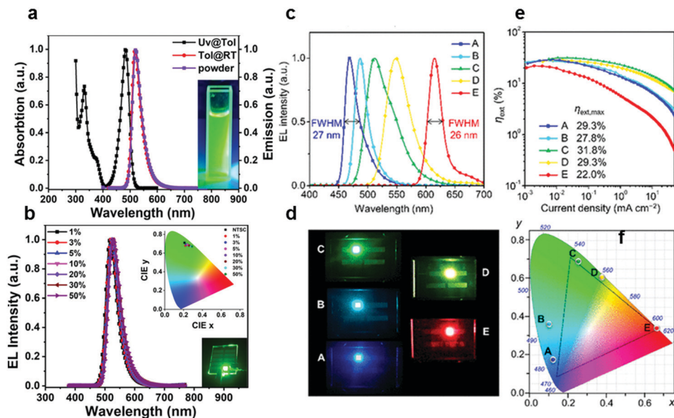
Fig. 8 (a) The normalized UV/Vis absorption and fluorescence spectra of m-Cz-BNCz measured in toluene solution and the corresponding powder fluorescence spectrum (inset: photograph in toluene taken under 365 nm UV light). (b) EL spectra of the devices (inset: the color coordinates of the devices and the photograph showing the emission color of the device at a 3 wt% doping concentration). Reprinted with permission from ref. 99. Copyright 2020 John Wiley and Sons; (c) EL characteristics of OLEDs (devices A–E) utilizing 1–5 as emitters. (d) EL spectra measured at 10 \text{ mA cm}^{-2} . (e) Photographs showing full-color EL emissions (left) and their EL color coordinates (right). (f) \eta_{\text{ext}} versus current density plots. Reprinted with permission from ref. 100. Copyright 2020 American Chemical Society.
