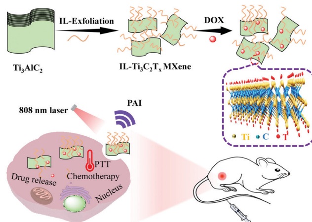
Scheme 1 Schematic illustration of the preparation of few-layer \text{Ti}_3\text{C}_2\text{T}_x MXene nanosheets with high chemical stability using an IL-assisted exfoliating method. The nanosheets can be used for photoacoustic imaging and the synergistic photothermal/chemotherapy of tumors.
