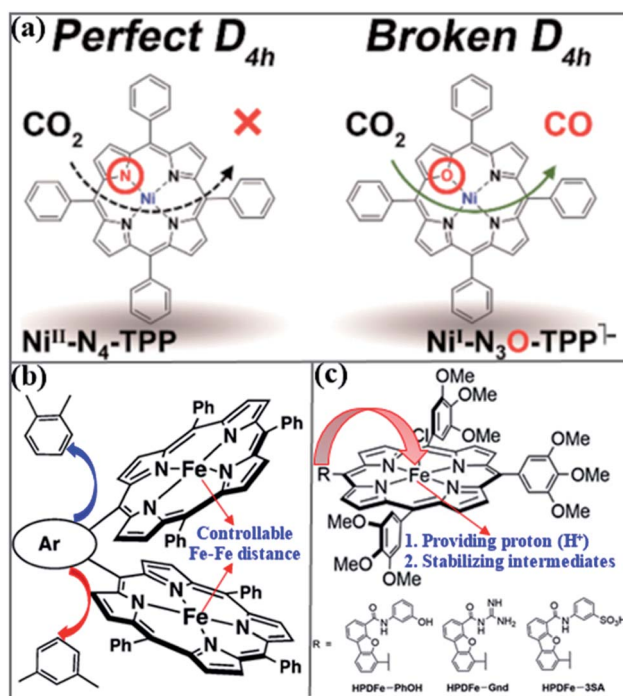
Fig. 8 (a) Concept principle of Ni-TPP complexes as CO_2 RR catalysts and one N ligated atom was changed into the O atom. Reprinted with permission from ref. 133. Copyright 2021, American Chemical Society. (b) Chemical structures of the iron porphyrin dimers, o -Fe 2 DTPP (above) and m -Fe 2 DTPP (below). Reprinted with permission from ref. 134. Copyright 2015, Royal Society of Chemistry. (c) The structure of hangman Fe porphyrins and the corresponding substituent groups. Reprinted with permission from ref. 135. Copyright 2018, American Chemical Society.
