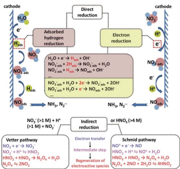
Fig. 8 The proposed reaction pathways for the \text{NO}_3\text{RR} . Reproduced with permission from ref. 121. Copyright 2021 The Royal Society of Chemistry.
