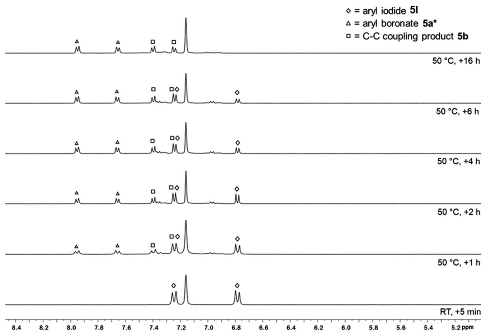
Fig. 5 In situ 1 H NMR spectra (aromatic region) of the reaction of the mono-NHC adduct \text{Me}_2\text{Im}^{\text{Me}} \cdot \text{B}_2\text{pin}_2 3 and 4-iodo-benzotrifluoride 5I in \text{C}_6\text{D}_6 at 50 °C (400 MHz). Diamond: 4-iodobenzotrifluoride 5I . Triangle: aryl boronic ester 5a (* in solution, the boron atom is coordinated by \text{Me}_2\text{Im}^{\text{Me}} forming the NHC adduct 5a-ADD ). Square: C–C coupling product 5b .
