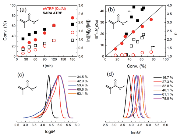
Fig. 6 (a) Kinetic plots, (b) evolution of M_n and \mathcal{D} vs. conv. during SARA ATRP (squares) or eATRP on a Cu/Al pair (circles) of MMA in EtOH + 0.05 M Bu 4 NCl, T = 50 °C. (c and d) Normalized evolution of molecular weight distribution of PMMA-Cl produced by SARA ATRP (c) or eATRP (d). Conditions: MMA/BPN/CuCl 2 /TPMA/Bu 4 NCl = 467/1/0.1/0.3/5, C MMA = 4.67 M. Full and empty symbols refer to the left and right ordinates, respectively. The black straight line represents M n th in (b).
