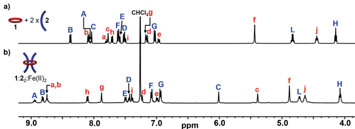
Fig. 2 Partial ^1\text{H-NMR} spectra of (a) 2 : 1 mixture of 2 : 1 (500 MHz, 25 °C, \text{CDCl}_3 ) and (b) 1 : 2 : \text{Fe(II)}_2 (500 MHz, 25 °C, 15% d_3 -MeCN in \text{CDCl}_3 ) after equilibration for 1 day at 45 °C. See Fig. 1 for the corresponding proton assignments.
