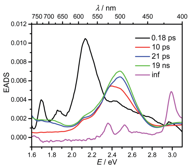
Fig. 5 Evolution associated difference spectra (EADS) from a global deconvolution of the transient absorption spectra of 1 in hexane at room temperature, excited at 333 nm (3.72 eV).
