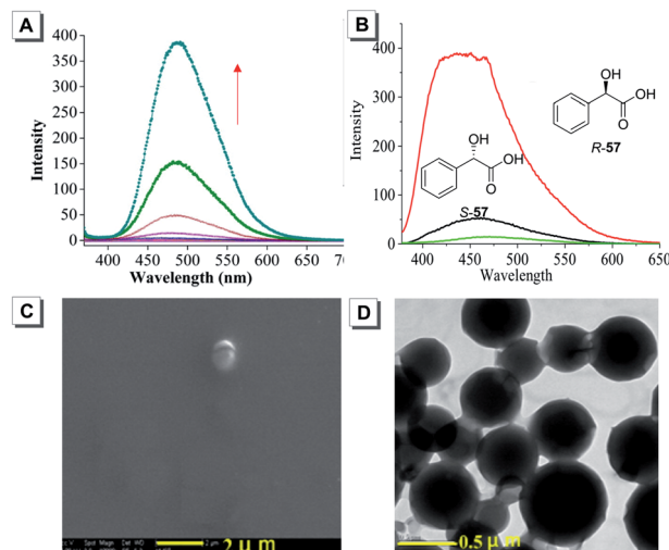
Fig. 23 (A) PL spectra of ( 1S,2S )- 7 in a mixture of THF and water with increasing water fraction. (B) PL spectra of ( 1S,2S )- 7 interacting with mandelic acid 57 . (C) SEM image of ( 1S,2S )- 7 with S - 57 . (D) TEM image of ( 1S,2S )- 7 with R - 57 . Adapted from ref. 54 with permission. Copyright 2015 American Chemical Society.
