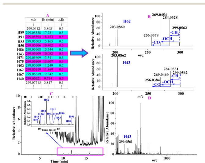
Fig. 6 An example of characterization flavonoids with low intensity. (A) In the constructed precursor ion list, twelve compounds ( H40 , H43 , H50 , H52 , H62 , H67 , H71 , H75 , H83 , H86 , H89 , and H91 ) were extracted at m/z 299.0556–299.0562; (B) performing targeted MS/MS analysis to obtain the fragmentation ions, such as H43 and H62 ; (C) the twelve compounds were covered by other high intensity ingredients and exhibited relative abundances of not more than 0.7% in a full scan; (D) the relative abundances of the precursor ions of these twelve ingredients were lower or much lower than those of others in MS spectra, such as H43 .
