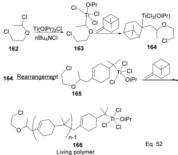
Scheme 46 Ti(OiPr) 3 Cl 3 -promoted cationic polymerization of β-pinene.
