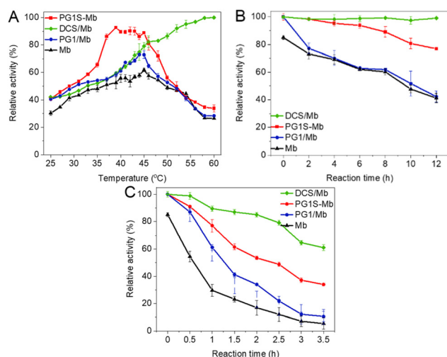
Fig. 6 Quantitative relative activity of Mb from different samples at different temperatures (A), as well as after being kept at (B) 25 ^{\circ}\text{C} and (C) 60 ^{\circ}\text{C} for different time intervals.
