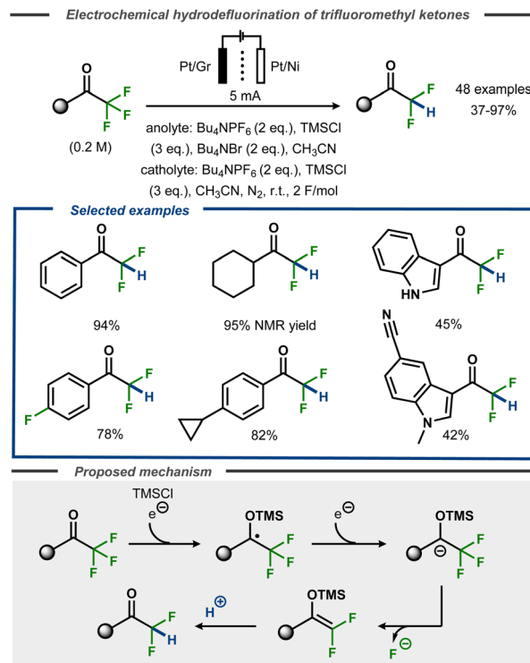
Fig. 23 Selective monoreduction of \alpha,\alpha,\alpha -trifluoromethyl ketones. 77
