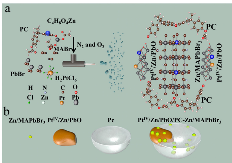
Scheme 1 The preparation of the \text{Pt}^{\text{IV}}/\text{Zn}/\text{PbO}/\text{PC-Zn}/\text{MAPbBr}_3 heterojunction materials. (a) A schematic illustration of the ESI-based microdroplet synthesis. (b) A schematic image of the structure.
