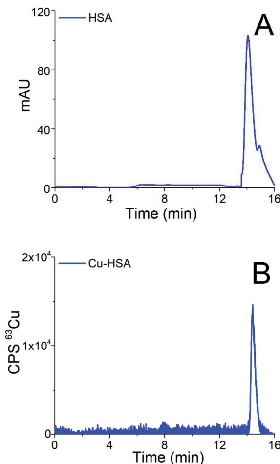
Fig. 2 Chromatograms of separation of the 15-times diluted sample of the standard serum protein HSA (25 g L -1 ) on the CLC monolithic column monitored by (A) UV detection (278 nm) and (B) ICP-MS detection at m/z 63.
