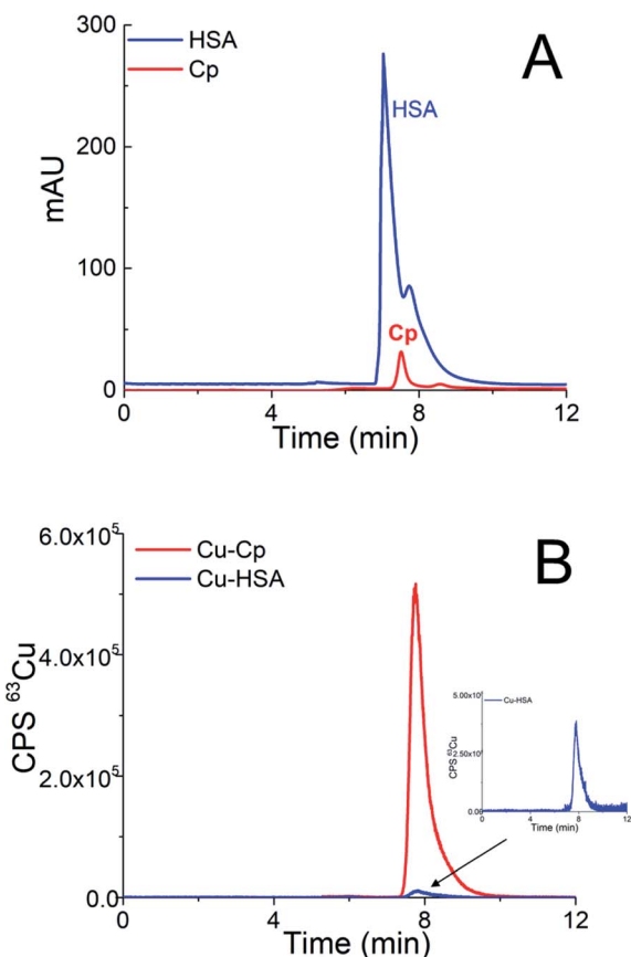
Fig. 1 Overlays of chromatograms of the 5-times diluted sample of a mixture of standard serum proteins HSA (25 g L -1 ) and Cp (1 g L -1 ) on the DEAE disk monitored by (A) UV detection (278 nm) and (B) ICP-MS detection at m/z 63.
