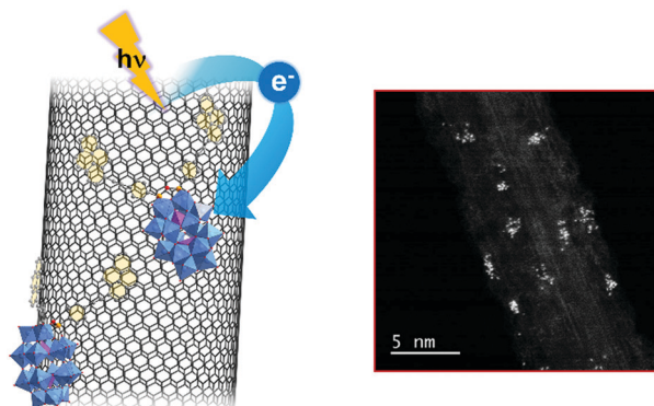
Fig. 28 (a) Non-covalent functionalisation of single-walled carbon nanotubes with a pyrene-functionalised Wells–Dawson oxocluster, highlighting the transient photo-driven charge transfer from the SWCNT to the appended POM complex, and: (b) HAADF-STEM imaging of the resultant nanocomposite (bright spots correspond to individual tungsten atoms in each POM). This figure has been adapted from ref. 209 with permission from the Royal Society of Chemistry, copyright 2014.
