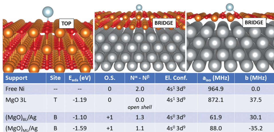
Fig. 6 Ni adatom. Most favourable adsorption mode on MgO 3L (left), (\text{MgO})_{\text{BL}}/\text{Ag} (middle) and (\text{MgO})_{\text{ML}}/\text{Ag} (right). Adsorption site (T = O top, B = bridge), adsorption energy ( E_{\text{ads}} ), formal oxidation state of the adatom (O.S.), number of unpaired electrons ( N^\alpha - N^\beta ), electron configuration (El. Conf.), and isotropic ( a_{\text{iso}} ) and anisotropic ( b ) hyperfine parameters.
