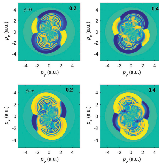
Fig. 15 The elliptic-dichroism parameter presented in false colors in the photoelectron momentum plane for ionization of Ar atoms by an \omega - 3\omega BEOTC field with ellipticity \varepsilon = 0.2 (left panels) and \varepsilon = 0.4 (right panels) and relative phase \phi = 0 (upper panels) and \phi = \pi (lower panels), corresponding to the spectra of Fig. 11 ( \phi = 0 ) and Fig. 13 ( \phi = \pi ). The false-color scale changes from -1 (blue) to +1 (yellow). The other laser parameters are as in Fig. 10.
