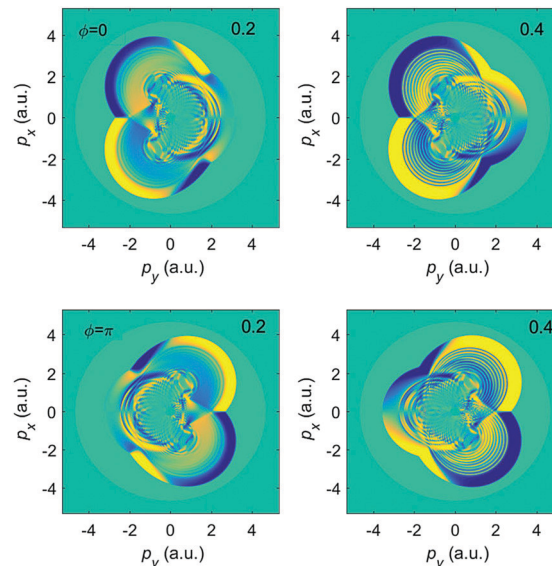
Fig. 14 The elliptic-dichroism parameter \delta(\mathbf{p}, \varepsilon) presented in false colors in the photoelectron momentum plane for ionization of Ar atoms by an \omega - 2\omega BEOTC field with ellipticity \varepsilon = 0.2 (left panels) and \varepsilon = 0.4 (right panels) and relative phase \phi = 0 (upper panels) and \phi = \pi (lower panels) corresponding to the spectra of Fig. 8 ( \phi = 0 ) and Fig. 12 ( \phi = \pi ). The false-color scale changes from -1 (blue) to +1 (yellow). The other laser parameters are as in Fig. 7.
