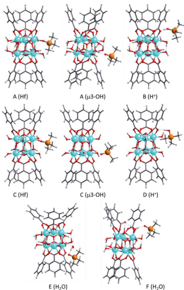
Fig. 5 Optimized geometries of TMPO interacting with Hf Lewis sites, \mu_3 -OH Brønsted acid sites, or additional H_2O molecules, and of protonated TMPOH^+ in Hf-MOF-808 models. The labels A to F identify the MOF-808 model used, as described in Fig. S1,† and the type of interaction between TMPO and MOF-808 is given in parenthesis. C and O atoms are depicted as gray and red sticks, Hf, P and H as cyan, yellow and white balls.
