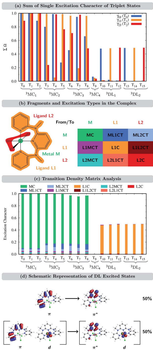
Fig. 3 (a) Sum of single excitation character \sum\Omega for the triplet states calculated from the transition density matrices \gamma_{0j} , \gamma_{1j} , and \gamma_{2j} of the T_0 , T_1 , and T_2 states, respectively. Note that \sum\Omega is set to 1 for \gamma_{II} to indicate that a state can be described quantitatively using itself as a reference when taking into account only single excitations. (b) Fragment partition and classification of excited-state characters in V^{III}Cl_3(ddpd) . (c) Transition density matrix analysis of the triplet states. Analysis used the transition-density matrix with the largest \sum\Omega out of \gamma_{0j} , \gamma_{1j} , and \gamma_{2j} . (d) Characterization of DL excited states.
