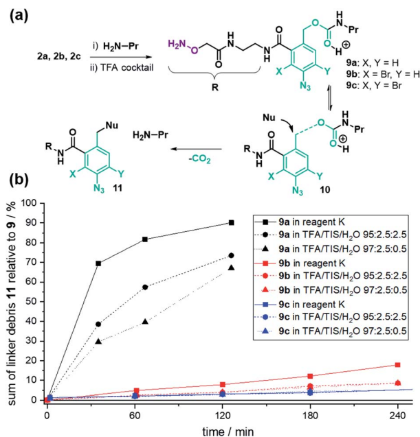
Fig. 2 (a) Generation of propylamine carbamates 9a-c from 2a-c . (b) TFA-stability analysis of carbamates 9a-c relative to the sum of UV-UPLC integrals of TFA-cleavage products 11 . reagent K: TFA/ \text{H}_2\text{O} /PhOH/PhSMe/ethanedithiol 82.5 : 5 : 5 : 5 : 2.4.
