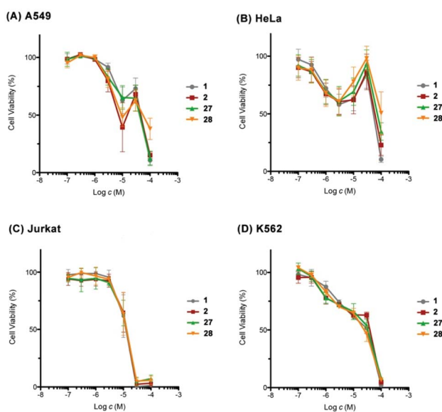
Fig. 3 Cytotoxic activity of synthetic amphirionin-2 ( 27 ) and its diastereomers 1 , 2 , and 28 . For an enlarged version of this figure, see Fig. S7, ESI.†
