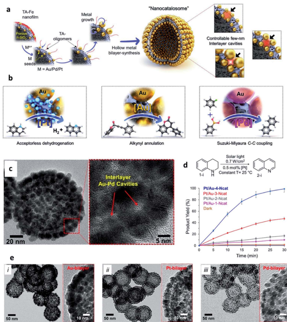
Fig. 9 (a) Schematic representation of the synthesis of metallic-bilayer Ncatal with controllable interlayer cavities of a few nm (right-side), with red shadows depicting change in interlayer cavity-structure; (b) catalytic applications of different Ncatal for different solar light induced reactions; (c) STEM images of the Pt/Au-1–4-Ncatal system; (d) [Pt]-catalysed dehydrogenation of THQ and conversion yields at different reaction times using Pt/Au-1–4-Ncatal; (e) TEM images of different metal bilayer nanocatalosomes [Au-4-Ncatal (i), Pt-Ncatal (ii), and Pd-Ncatal (iii)]. Reproduced with permission from ref. 98. Copyright 2020 Wiley and Sons.
