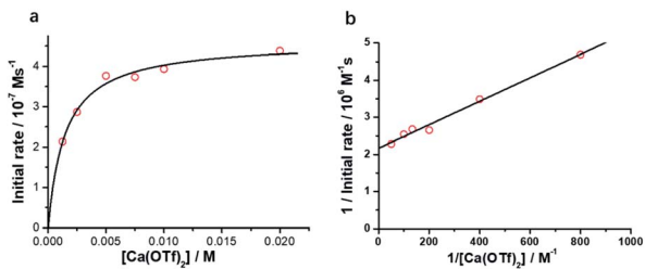
Fig. 3 Effects of [\text{Ca}(\text{OTf})_2] on cyclohexane oxidation by \text{RuO}_4^- in \text{CH}_3\text{CN} . Conditions: [\text{Pr}_4\text{N}][\text{RuO}_4] (0.01 M), cyclohexane (1.0 M) in \text{CH}_3\text{CN} at 23 °C. (a) Plot of initial rate vs. [\text{Ca}(\text{OTf})_2] . (b) Plot of 1/\text{initial rate} vs. 1/[\text{Ca}(\text{OTf})_2] (slope = (3.16 \pm 0.15) \times 10^3 , y-intercept = (2.16 \pm 0.06) \times 10^6 , r = 0.988 ).
