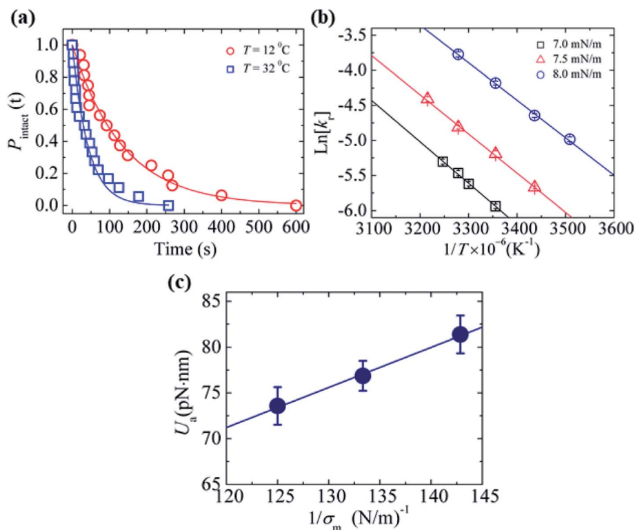
Fig. 10 The effects of temperature on the constant-mechanical-tension ( \sigma_m )-induced rupture of DOPC-GUVs. (a) The time-dependent P_{\text{intact}}(t) values at temperatures of T = 12\text{ }^\circ\text{C} ( \circ ) and T = 32\text{ }^\circ\text{C} ( \square ) at \sigma_m = 8.0\text{ mN m}^{-1} . The solid lines represent the best fit curves based on eqn (4). (b) The relationship between \ln k_f and 1/T at \sigma_m = 7.0\text{ mN m}^{-1} ( \square ), 7.5\text{ mN m}^{-1} ( \Delta ), and 8.0\text{ mN m}^{-1} ( \circ ). Average values of k_f with standard error for each temperature were determined using three independent experiments, each of which was performed using 20 GUVs for each tension. The solid lines show the best linear fits. (c) The relationship between U_a and 1/\sigma_m . The error bars show standard error. The solid line indicates the best fit curve using eqn (10). The images in a–c have been adapted from ref. 101 with permission from AIP Publishing LLC, copyright 2015.
