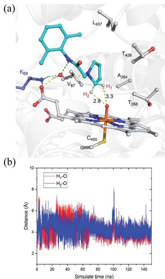
Fig. 1 (a) QM(UB3LYP/B1)/MM optimized structure of the Cpd I with the bound substrate, pyrrolidine derivative of lidocaine, taken from a representative snapshot in the equilibrated MD trajectory. Key distances are given in angstroms. Most hydrogen atoms of C–H bonds have been omitted for clarity. (b) Distance fluctuations between Cpd I -O and the H 1 atom (red), the H 2 atom (blue) of the substrate throughout the MD trajectory.
