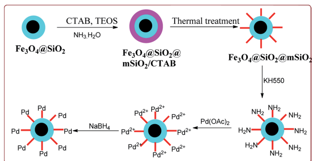
Scheme 9 Preparation of immobilized \text{Fe}_3\text{O}_4@SiO_2@mSiO_2 -Pd(0) nanocatalyst.
