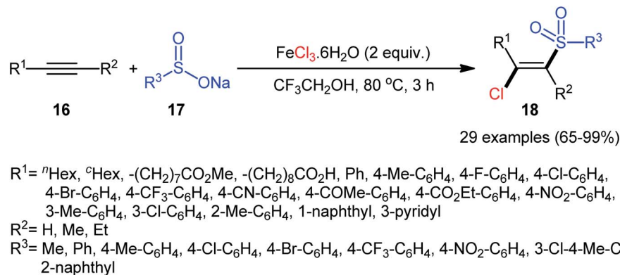
Scheme 8 Synthesis of ( E )-β-chlorovinyl sulfones 18 via three-component reaction between alkynes 16 , sodium sulfinates 17 and FeCl_3 \cdot 6H_2O .
