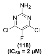
Fig. 32 Chemical structure of a selected 5-substituted 2-amino-4,6-dihydroxypyrimidine (118).
