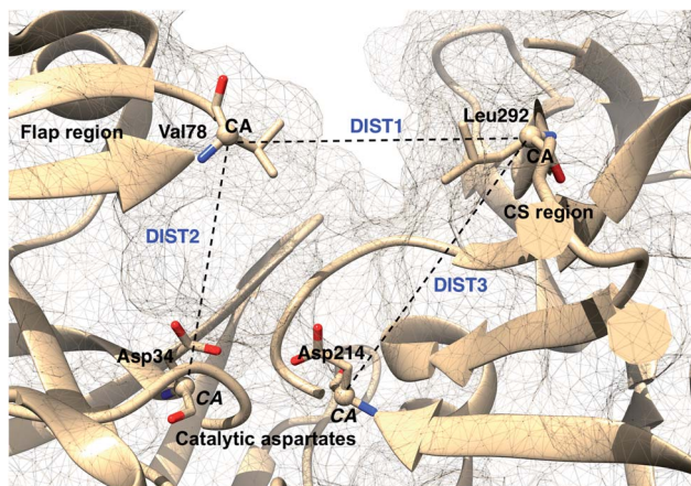
Fig. 5 Different distance based order parameters proposed by Karubi et al. DIST2 measures the extent of flap opening whereas DIST3 accounts for opening of CS region. Fig. 12 shows that DIST2 and DIST3 are uncorrelated which gives an indication that in apo PAPs, the dynamics of flap and CS region are independent of each other. DIST1 acted as an auxiliary order parameter. These distance based order parameters can be generalised for other PAPs. The image was created using PDB:1LF4.
