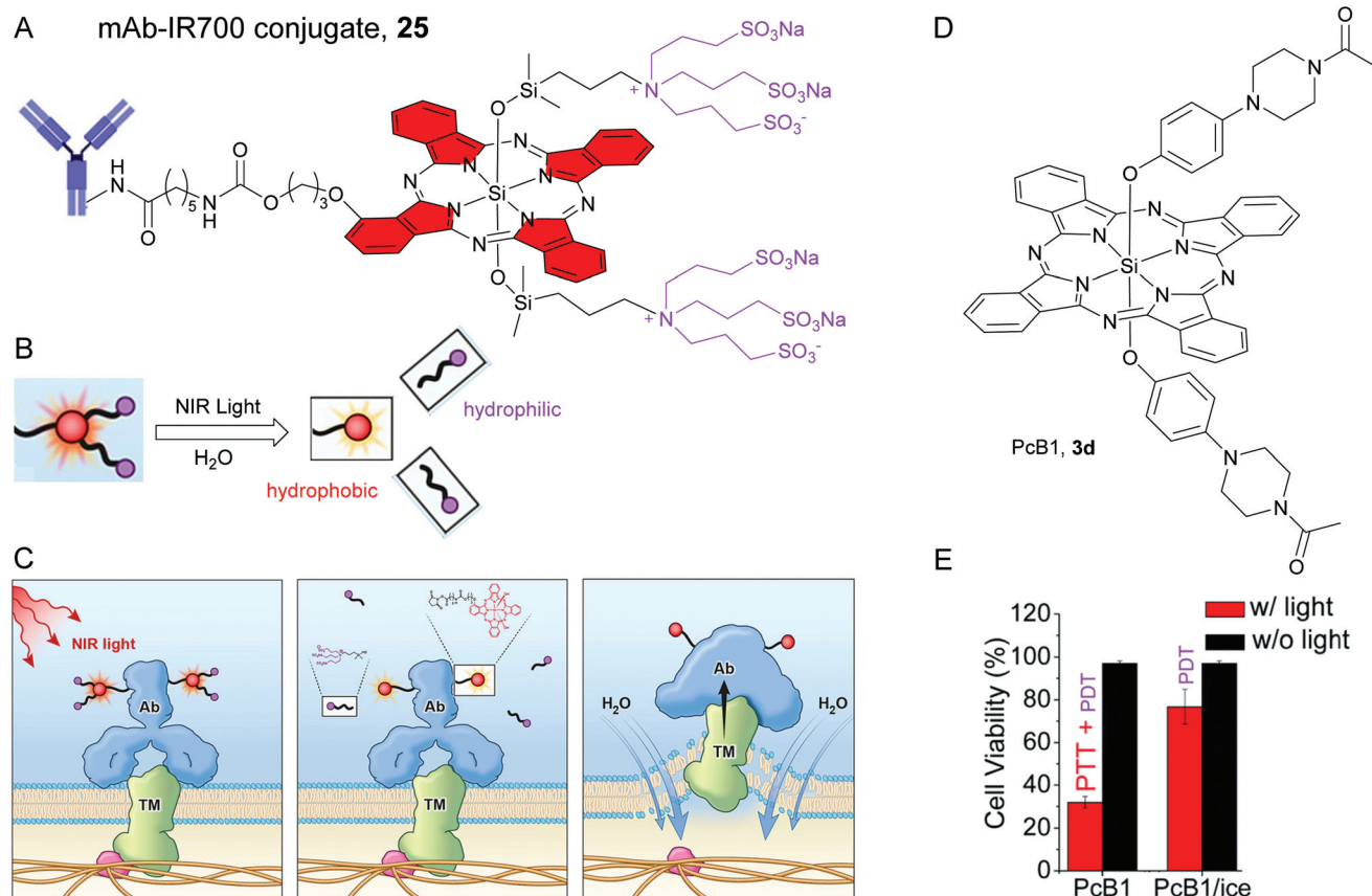
Fig. 6 (A) Structure of mAb-IR700 conjugate, 25 . The red colour is used to highlight the hydrophobic SiPc core rings and the violet colour is used to highlight the hydrophilic axial ligands. (B) NIR light induced decomposition of the SiPc molecule attached to the antibody. NIR light irradiation causes mAb-IR700 to release the hydrophilic ligand (violet circles), which makes mAb-IR700 hydrophobic and causes aggregation. (C) Scheme indicates the proposed mechanism of NIR-PIT. An antibody-IR700-antigen complex is formed on the cell membrane. With NIR light irradiation, the ligands of IR700 were released from the antibody-IR700-antigen complex. The physical changes in aggregation and solubility of the antibody-IR700-antigen complex may produce physical stress on the membrane locally impairing cellular membrane function for maintaining membrane pressure, and then the water outside of the cell was flown into the cell to burst the cell. Reproduced with permission from ref. 18. Further permissions related to the material excerpted should be directed to the ACS ( https://pubs.acs.org/doi/10.1021/acscentsci.8b00565 ). (D) Chemical structure of SiPc, 3d or PcB1. (E) Cytotoxic effect of 3d or PcB1 on HepG2 cells with (red bars) and without (black bars) laser irradiation. PcB1/ice mean controlling the temperature of cells at below 30 °C via an ice-bath during laser treatment. Reproduced from ref. 110 with permissions from Royal Society of Chemistry.
