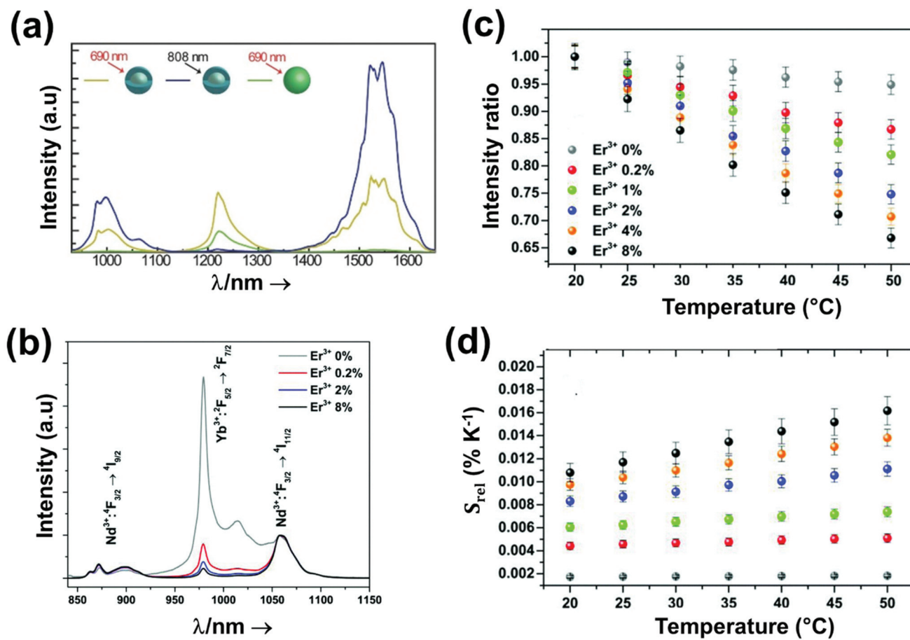
Fig. 28 (a) Room temperature emission spectra of simple core Er^{3+}, Tm^{3+}, Yb^{3+}:LaF_3 under 690 nm excitation (green) and of active core@active shell Er^{3+}, Yb^{3+}:LaF_3@Yb^{3+}, Tm^{3+}:LaF_3 (concentrations of lanthanide ions Tm^{3+}, Yb^{3+} and Er^{3+} are 10 mol%, 10 mol% and 2 mol%, respectively) under 690 (yellow) and 808 nm (blue) laser excitation. The green sphere and the grey core covered with a blue sphere represent the simple core and the active core@active shell, respectively. Reprinted with permission from ref. 240. Copyright 2017, Wiley-VCH Verlag GmbH & Co. KGaA. Effect of the Er^{3+} concentration on: (b) the intensity of the emissions, (c) the intensity ratio, and (d) S_{rel} on Tm^{3+}, Yb^{3+}:SrF_2@Y^{3+}:SrF_2@Er^{3+}, Nd^{3+}, Yb^{3+}:SrF_2@Nd^{3+}:SrF_2 nanocrystals. (b)–(d) Adapted with permission from ref. 242. Copyright 2018, The Royal Society of Chemistry.
