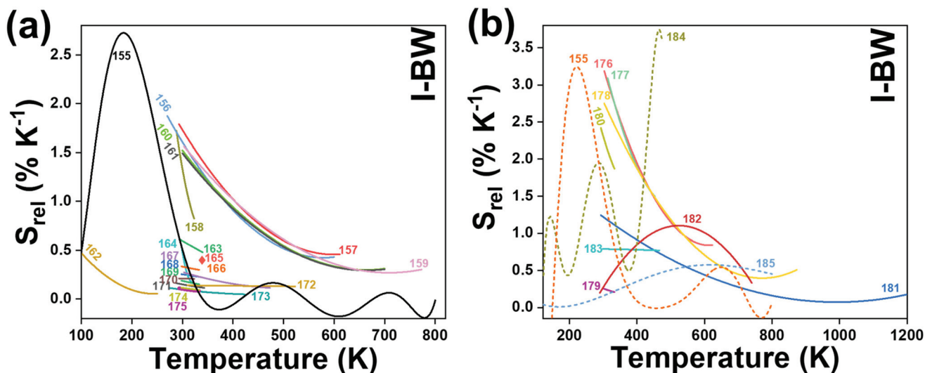
Fig. 15 Temperature dependence of S_{\text{rel}} for: (a) single doping and (b) codoping with other lanthanide ions (in solid lines) and transition metal ions (in dashed lines) for \text{Nd}^{3+} luminescent thermometers, operating in the I-BW. The numbers represent the corresponding references for each \text{Nd}^{3+} -based thermometer.
