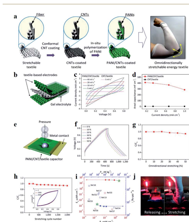
Fig. 1 (a) Synthetic procedure of PANI/CNT. (b) Device configuration of electrochemical capacitors assembled from the textile-based electrode and gel electrolyte. (c) Cyclic voltammetry curves of textile-based electrochemical capacitors under different scan rates. (d) Areal-specific capacitance vs. current density. (e) Schematic illustration of evaluation method for omnidirectional stretchability of PANI/CNT/textile capacitor. (f) Galvanostatic charge/discharge curves at various omnidirectional stretching levels. (g) Capacitance retention under omnidirectional stretching levels. (h) Cycle stability of PANI/CNT/textile capacitors under repeated 20% omnidirectional stretching level. (i) Ragone plot with the previously reported stretchable electrochemical capacitors. (j) LED lighting powered by PANI/CNT/textile capacitors under finger pressure. Reproduced with permission. 14 Copyright 2019, American Chemical Society.
