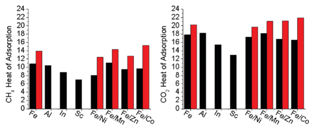
Fig. 6 The average heat of adsorption for CH 4 and CO 2 for the micro-porous (black) and mesoporous (red) sample isomorphs. Heat of adsorption was calculated based on the experimental adsorption isotherms at 195 K, 273 K, and 298 K for each gas.
