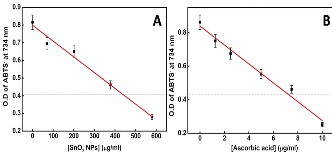
Fig. 13 (A) Plot of [SnO 2 NPs] vs. OD of the ABTS radical at 734 nm. (B) Plot of [ascorbic acid] vs. OD of the ABTS radical at 734 nm.
