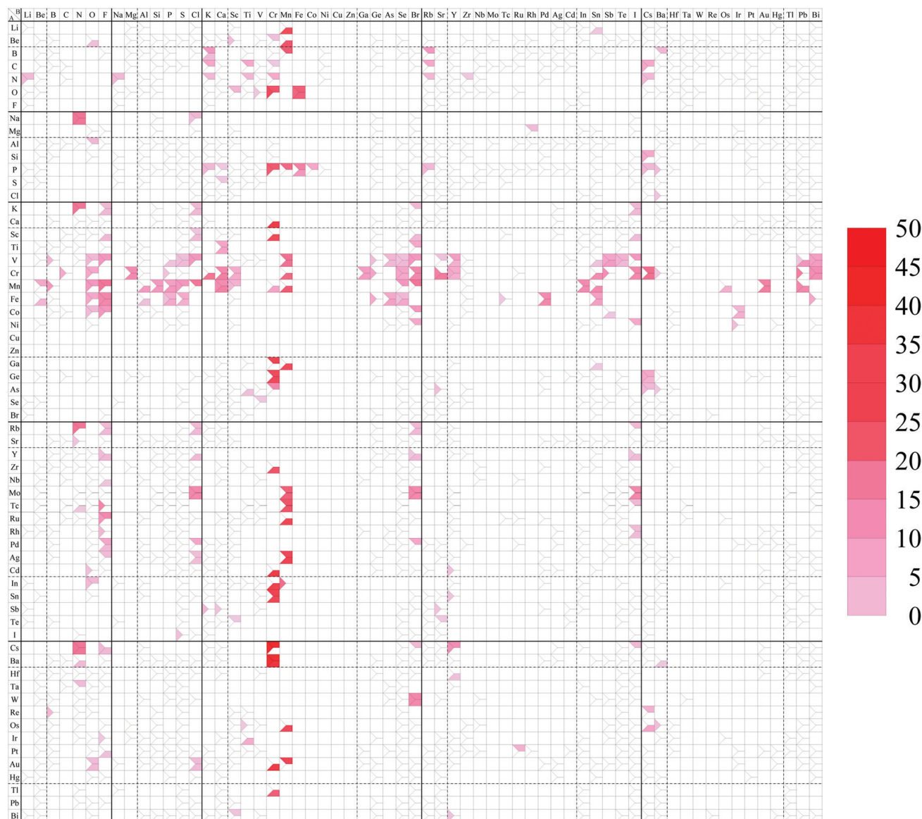
Fig. 11 Spin magnetic moment map for AB_2 type monolayers. The degree of intensity of red color represents the magnitude of the spin magnetic moment [ \mu_B per unit cell].
