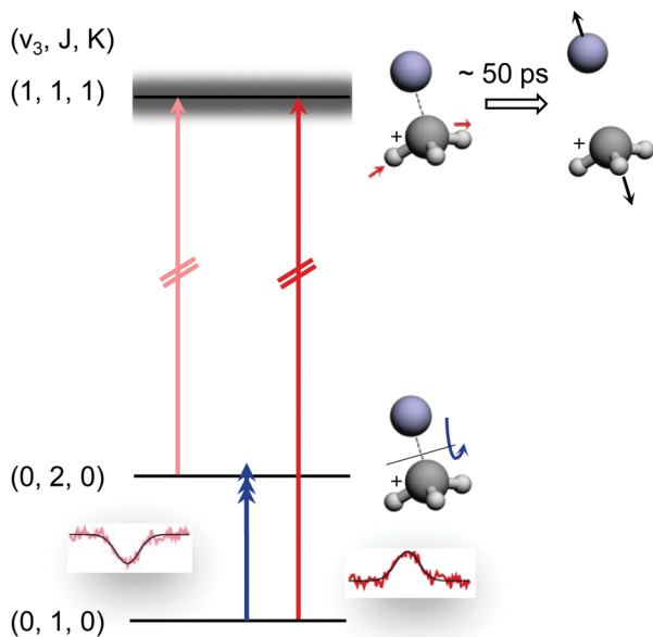
Fig. 11 Rotational-predissociation double resonance scheme illustrated for the example of \text{CH}_3^+-\text{He} . 28 The fixed IR laser probes either the initial (dark red) or the final (light red) level of the rotational transition (blue), giving rise to different signal forms when the frequency of the rotational excitation is scanned: in the left combination, the rotational transition pumps ions into the level (0,2,0) probed by the IR laser, enhancing the dissociation of \text{CH}_3^+-\text{He} . In the right combination, the rotational transition pumps ions out of the level (0,1,0) probed by the IR laser, thus hindering the dissociation. Reprinted with permission of APS.
