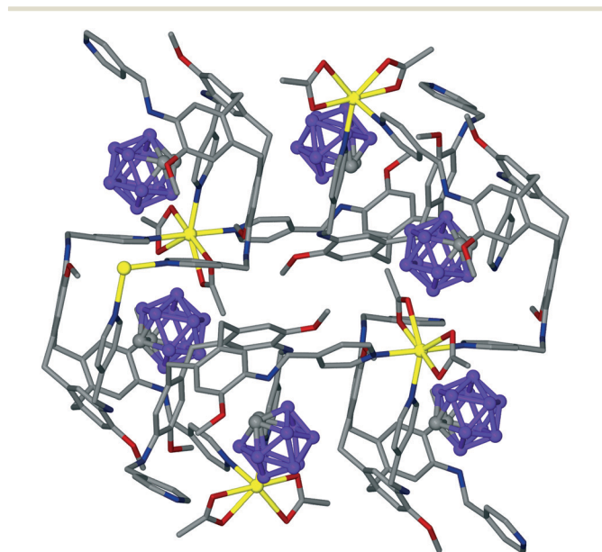
Fig. 2 Section of the crystal structure of [Cd(L5)(OAc) 2 ] showing formation of 2D network and host-guest binding of C 2 B 10 H 12 o-carborane guests (purple). Hydrogen atoms excluded. 14
