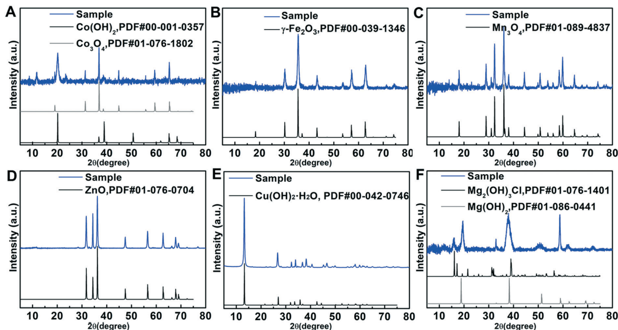
Fig. 1 XRD patterns of the ultrathin two-dimensional metal oxide and hydroxide nanosheets: (A) \text{Co}_3\text{O}_4/\text{Co}(\text{OH})_2 , (B) \gamma\text{-Fe}_2\text{O}_3 , (C) \text{Mn}_3\text{O}_4 , (D) \text{ZnO} , (E) \text{Cu}(\text{OH})_2\cdot\text{H}_2\text{O} and (F) \text{Mg}(\text{OH})_2/\text{Mg}_2(\text{OH})_3\text{Cl} .
