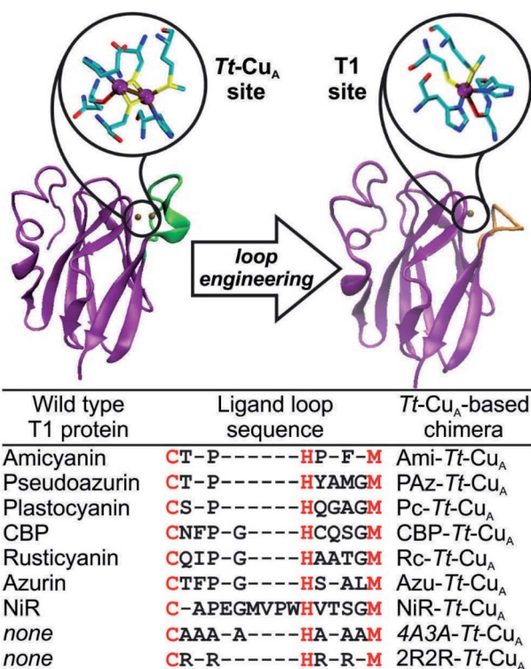
Fig. 1 X-ray crystallographic structures of native Tt -Cu A (PDB ID 2CUA) 38 on the left, and that of Ami - Tt -Cu A on the right (PDB ID 5U7N). 36 The loop replaced in the chimeras is indicated in green and orange, respectively. The loop sequences employed to obtain the different chimeras are listed below. Red letters denote the conserved ligand set.
