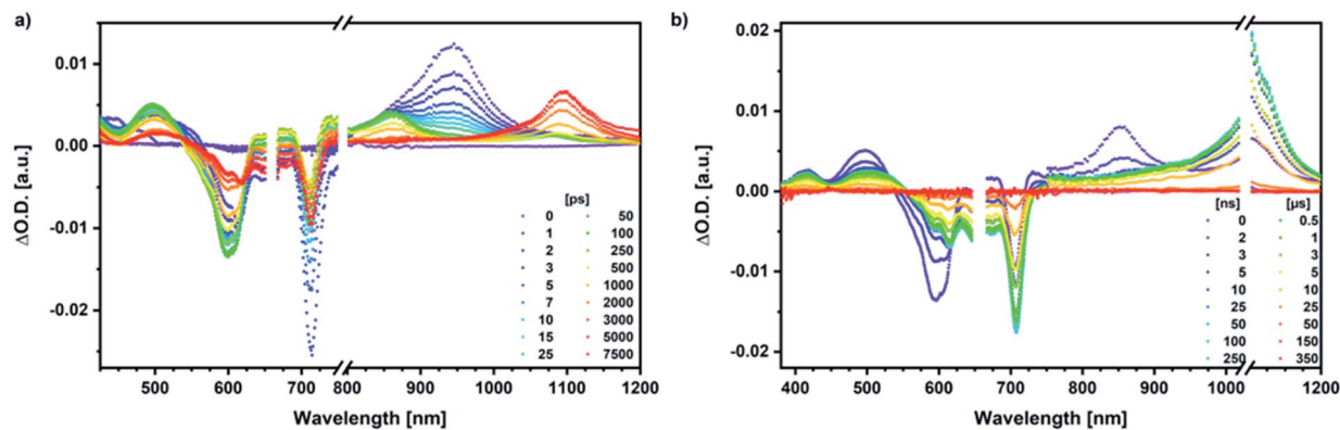
Fig. 12 (a) Femtosecond differential absorption spectra of syn -SubPc 1 (1.5 × 10 -5 M) and \text{C}_{60} (3.0 × 10 -4 M) in argon purged chlorobenzene at delay times between 0 and 7500 ps after 656 nm laser excitation (200 nJ) at room temperature. (b) Nanosecond differential absorption spectra of syn -SubPc 1 (1.5 × 10 -5 M) and \text{C}_{60} (3.0 × 10 -4 M) in argon purged chlorobenzene with delay times between 0 and 350 μs after 656 nm laser excitation (450 nJ) at room temperature.
