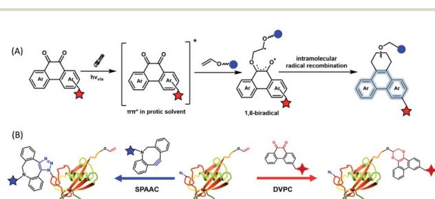
Fig. 2 (A) Visible-light driven bioorthogonal dione–vinyl ether photocycloaddition (DVPC) reaction via the PeT pathway; (B) orthogonal protein labelling achieved by SPAAC and DVPC that are orthogonal to each other.
