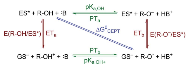
Scheme 1 ES-PCET reaction diagram. ES* is the excited sensitizer, GS - is the reduced sensitizer, R-OH is the protonated substrate, and B is a base.
