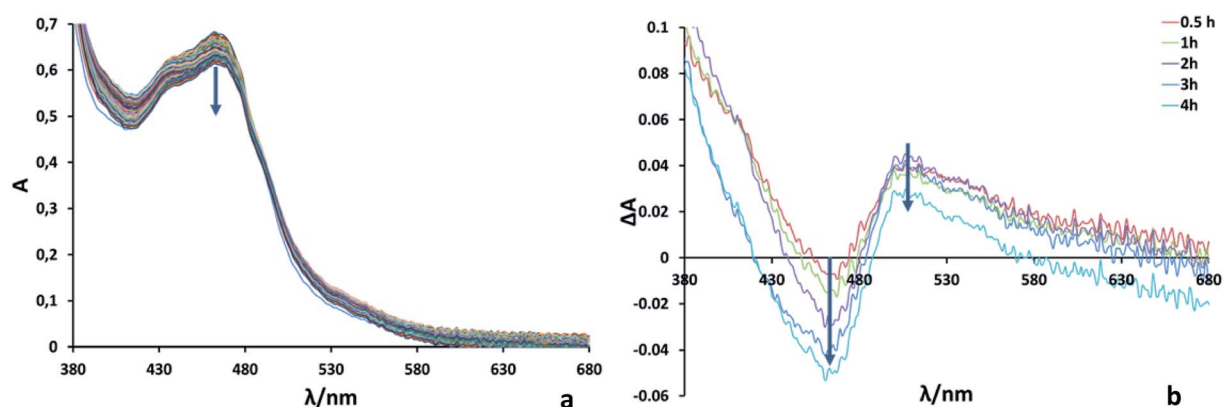
Fig. 3 (a) UV-vis absorption spectra during irradiation of a DMA-TEOA (5 : 1 v/v) solution containing RuRe2 (50 μM) and BIH (0.1 M) at λ ex = 480 nm for 240 min at 1 min intervals. (b) UV-vis differential absorption spectra between before and after irradiation.
