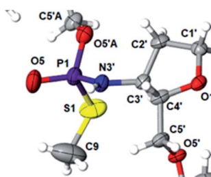
Fig. 1 Crystal structure of {}^{\text{DMT}}dG^{\text{iBu}}_{\text{NPSMe}}T_{\text{OAc}} 10f showing partial structure and spatial orientation of substituents around the phosphorus stereogenic center (marked P1). Compound 10 was obtained from the monomer 6Gf (fast-eluting 5'- O -DMT-3'-amino-2',3'-dideoxy- N 6- i Bu-guanosine-3'- N -(2-thio-4,4-pentamethylene-1,3,2-oxathiaphospholane). The oxygen atom marked O5'A belongs to the thymidine residue.
