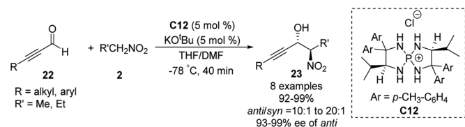
Scheme 33 Catalytic asymmetric direct Henry reaction of ynals.
