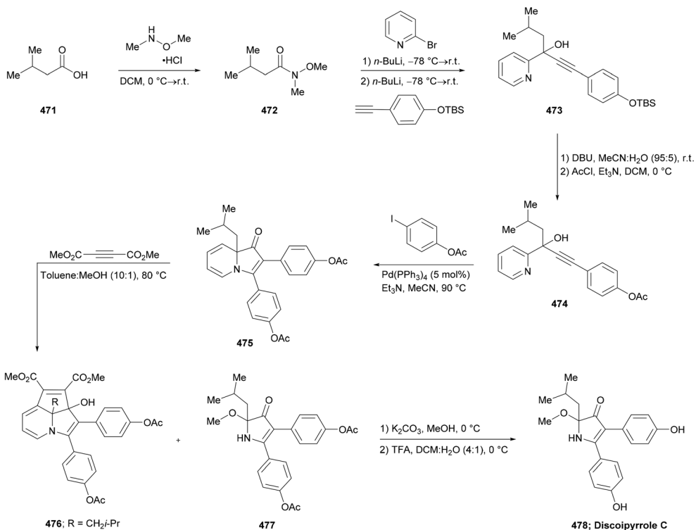
Scheme 112 Synthesis of discoipyrole C.
