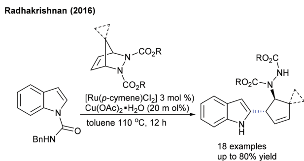
Scheme 73 C2-Functionalization of indoles with heterobicyclic alkenes.
