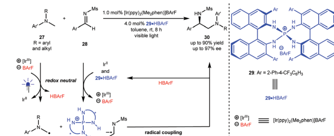
Scheme 8 Redox neutral \alpha -coupling of N -arylaminoethanes with aldimines.
